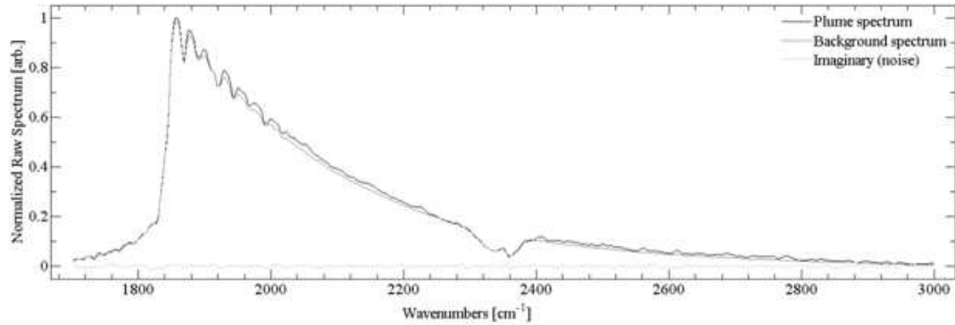
Figure 48. Spectrum associated with the detonation of MeS. The circle in Figure 10 marks the time step associated with the plume spectrum, which corresponds to the localized peak of normalized radiance. This plume spectrum is overlaid with the background spectrum and the instrument noise.
