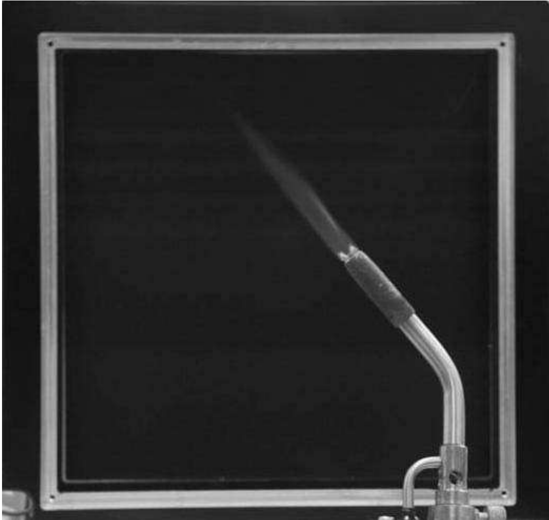
Figure 6. Experimental Setup to collect propane torch spectra. The propane torch was locked in place directly in front of a blackbody background source at 65°C. The FIRST-MWE was set to a spectral resolution of 16cm -1 and windowed to a spatial view of 128x128 pixels. Data was collected in both spectral and camera modes.
