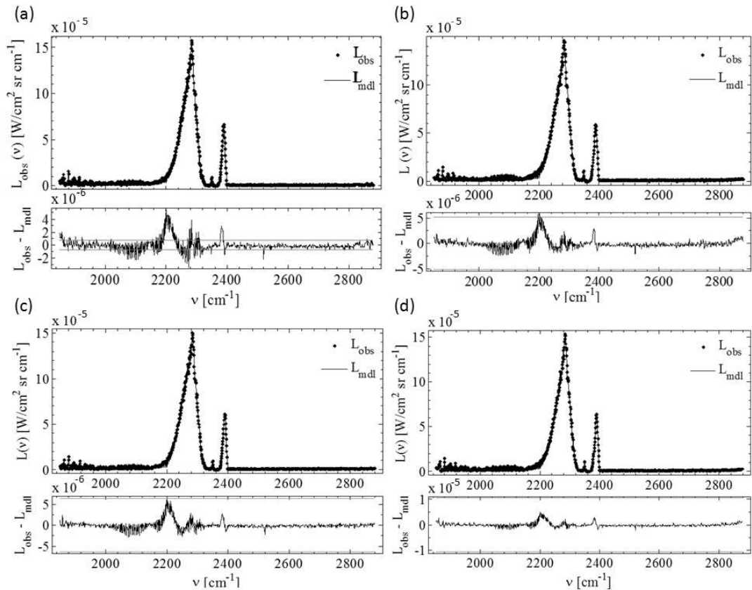
Figure 52. Results from fitting jet engine exhaust data to single-temperature plume model for the hottest region of the plume. (a) Diesel fuel with flow rate of 300 \frac{\text{cm}^{-3}}{\text{min}} . (b) Diesel fuel with flow rate of 150 \frac{\text{cm}^{-3}}{\text{min}} . (c) Kerosene fuel with flow rate of 300 \frac{\text{cm}^{-3}}{\text{min}} . (d) Kerosene fuel with flow rate of 150 \frac{\text{cm}^{-3}}{\text{min}} .
